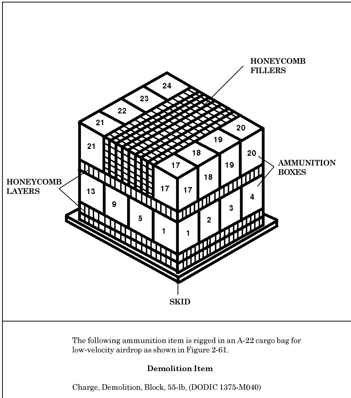
Figure 2-61. Ammunition Layout in an A-22 Cargo Bag for Low-Velocity Airdrop
