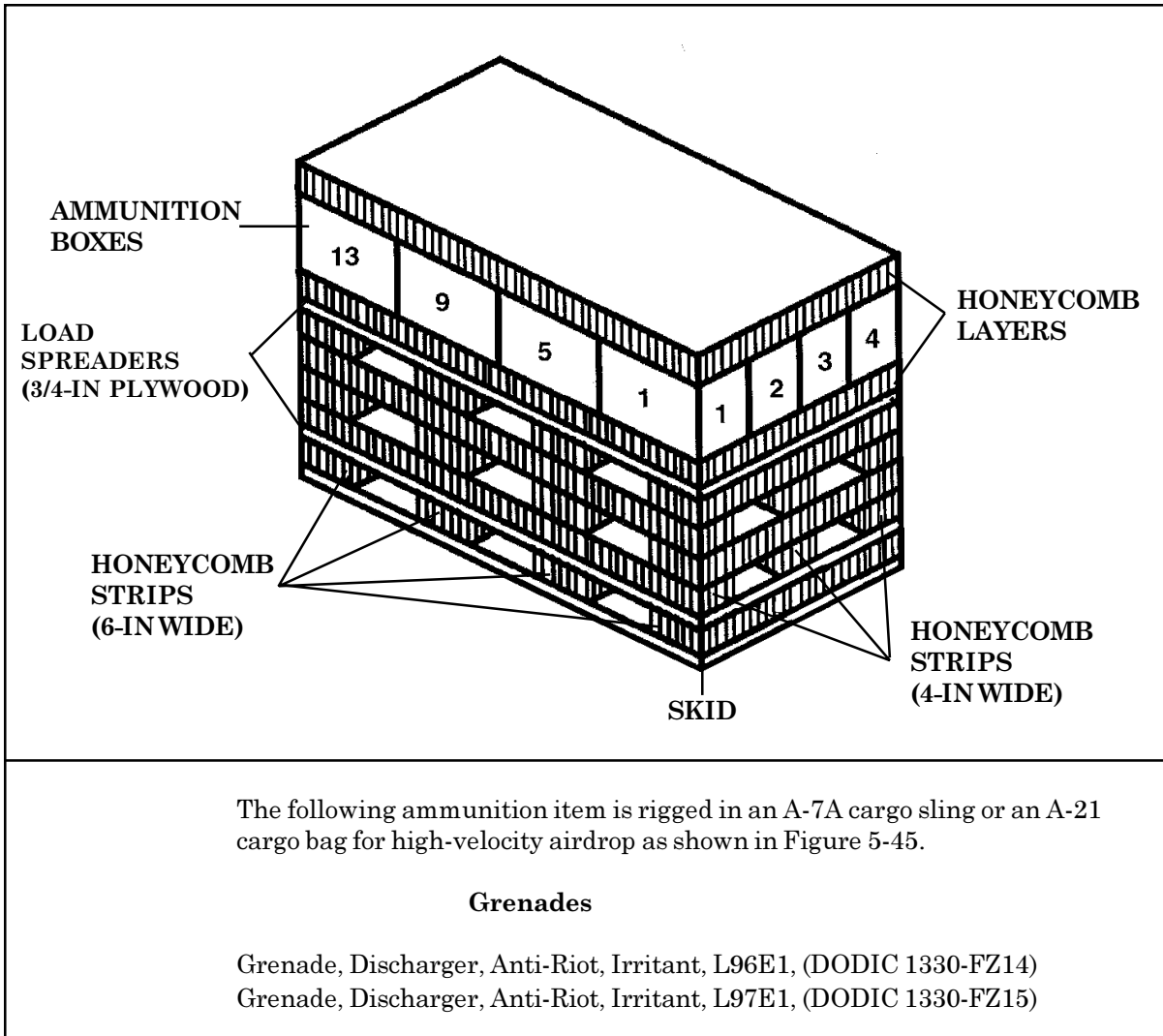
Figure 5-45. Ammunition Layout in an A-7A Cargo Sling or an A-21 Cargo Bag for High-Velocity Airdrop
