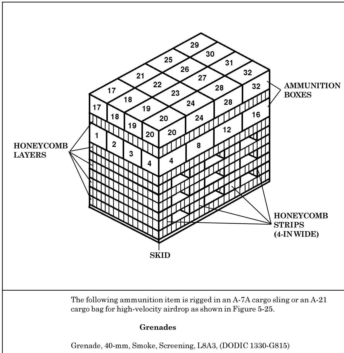
Figure 5-25. Ammunition Layout in an A-7A Cargo Sling or an A-21 Cargo Bag for High-Velocity Airdrop
