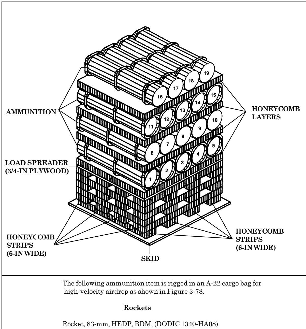
Figure 3-78. Ammunition Layout in an A-22 Cargo Bag for High-Velocity Airdrop
