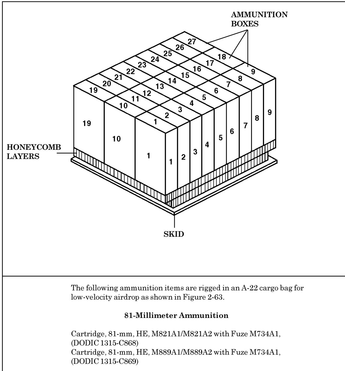
Figure 2-63. Ammunition Layout in an A-22 Cargo Bag for Low-Velocity Airdrop
