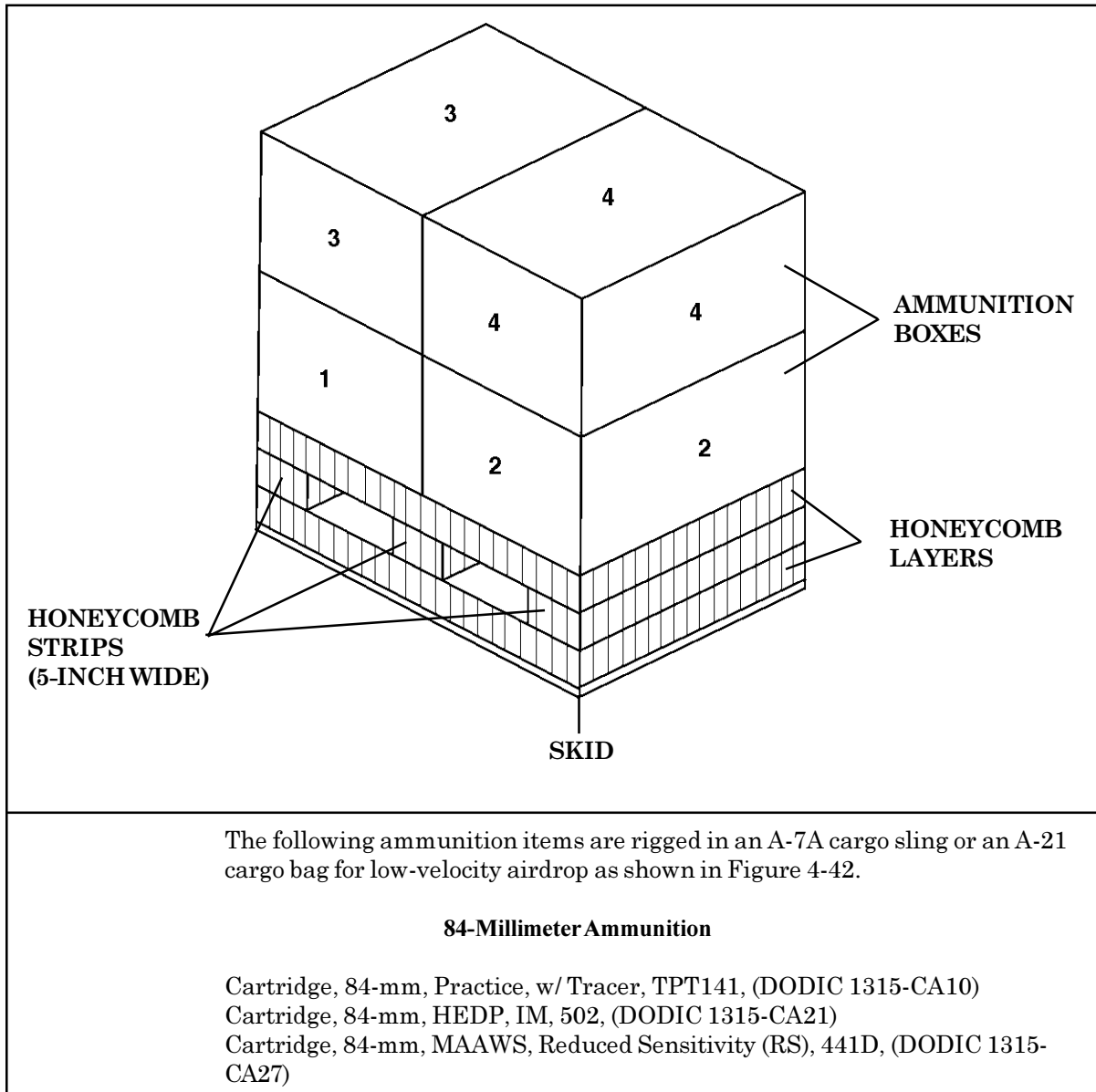
Figure 4-42. Ammunition Layout in an A-7A Cargo Sling or an A-21 Cargo Bag for Low-Velocity Airdrop
