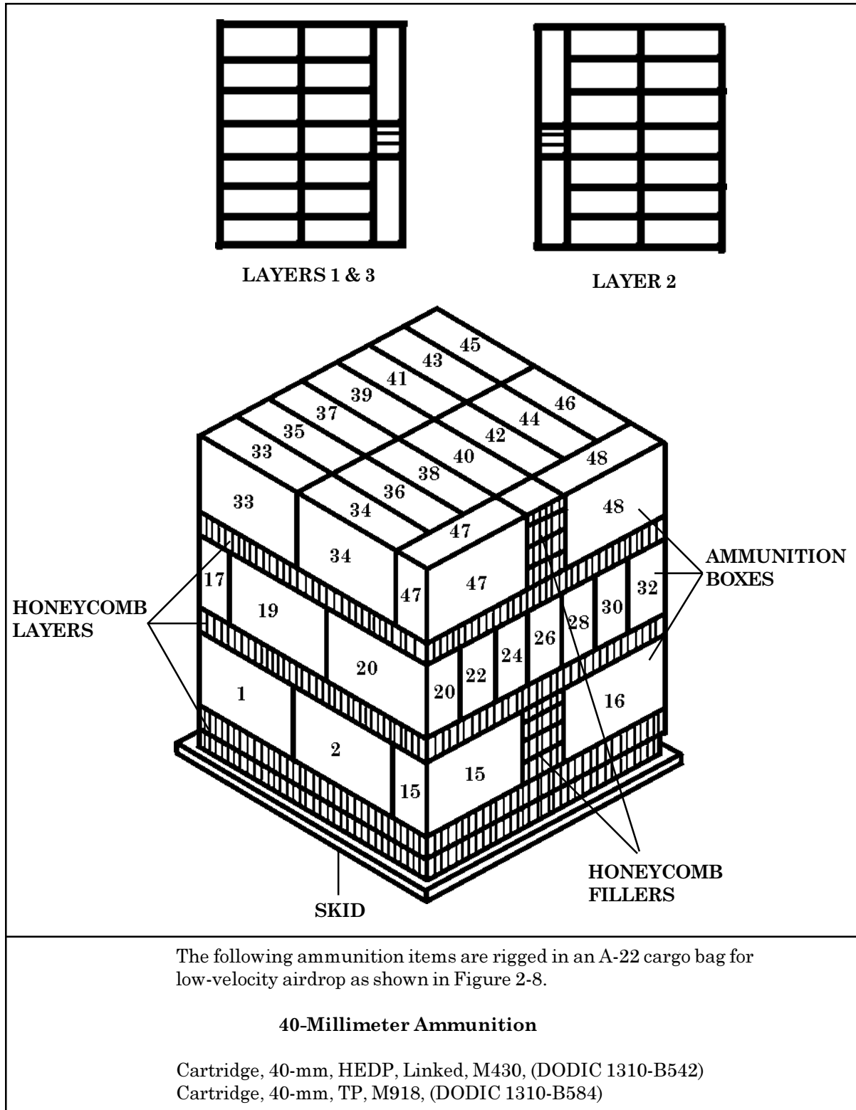
Figure 2-8. Ammunition Layout in an A-22 Cargo Bag for Low-Velocity Airdrop
