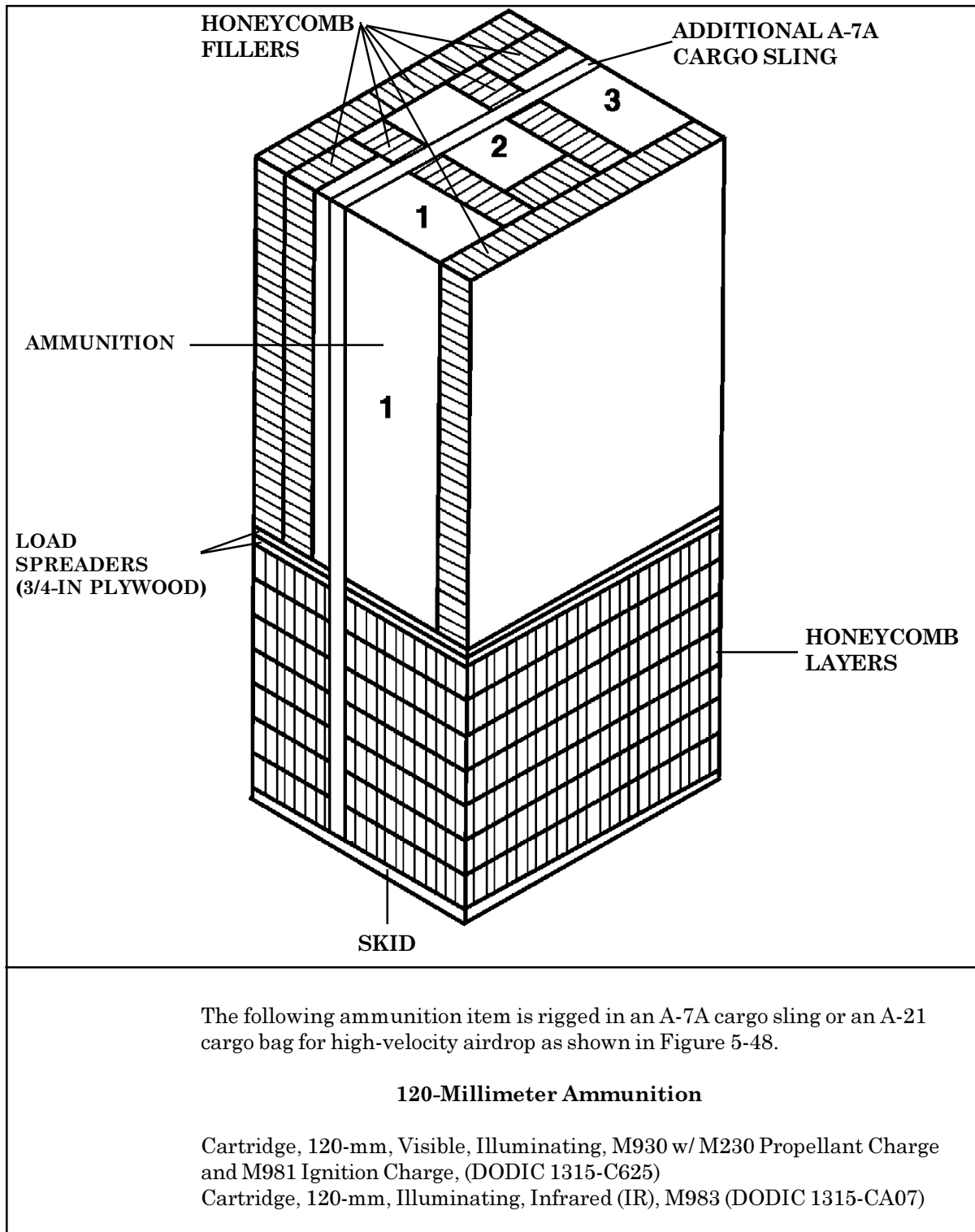
Figure 5-48. Ammunition Layout in an A-7A Cargo Sling or an A-21 Cargo Bag for High-Velocity Airdrop
