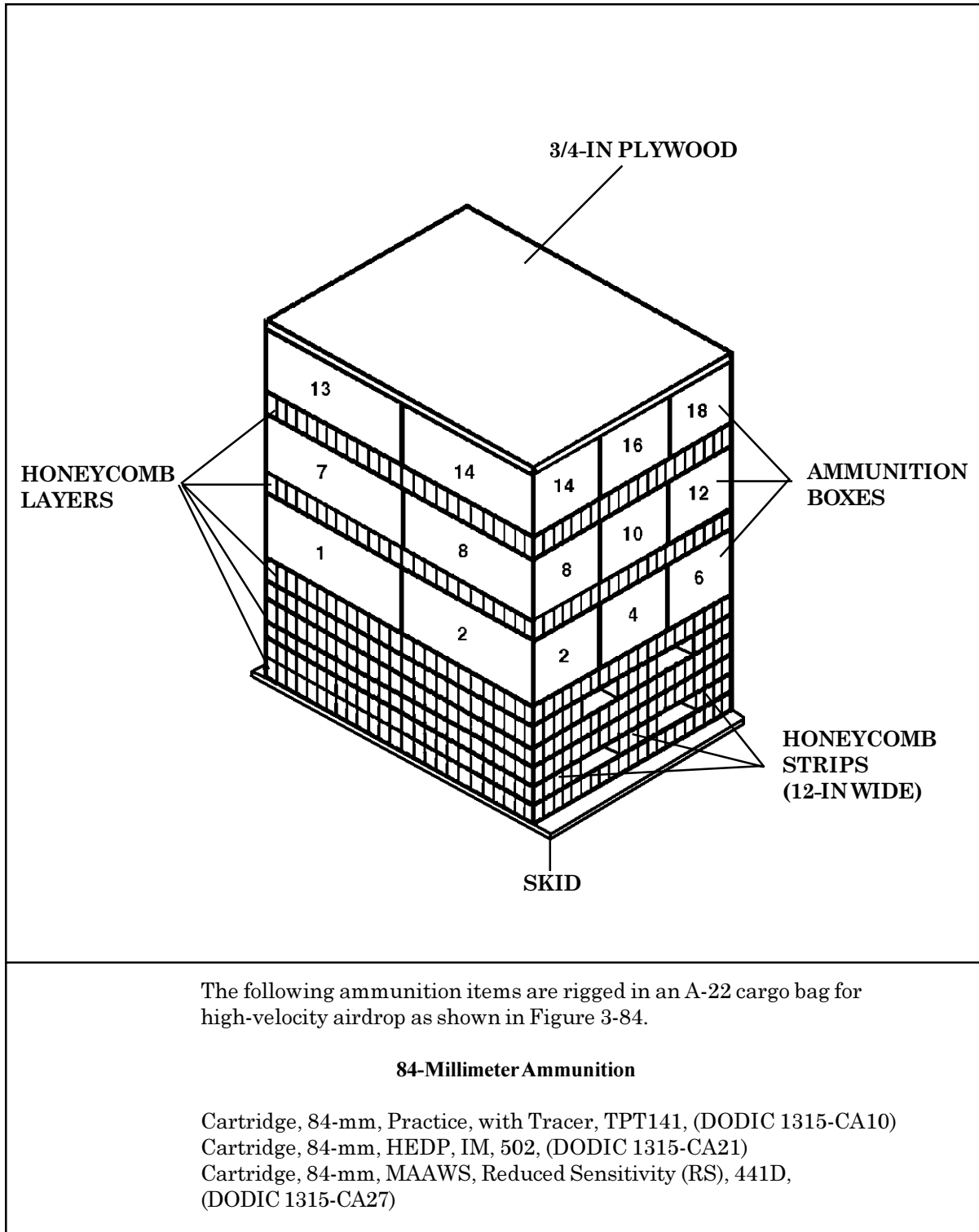
Figure 3-84. Ammunition Layout in an A-22 Cargo Bag for High-Velocity Airdrop
